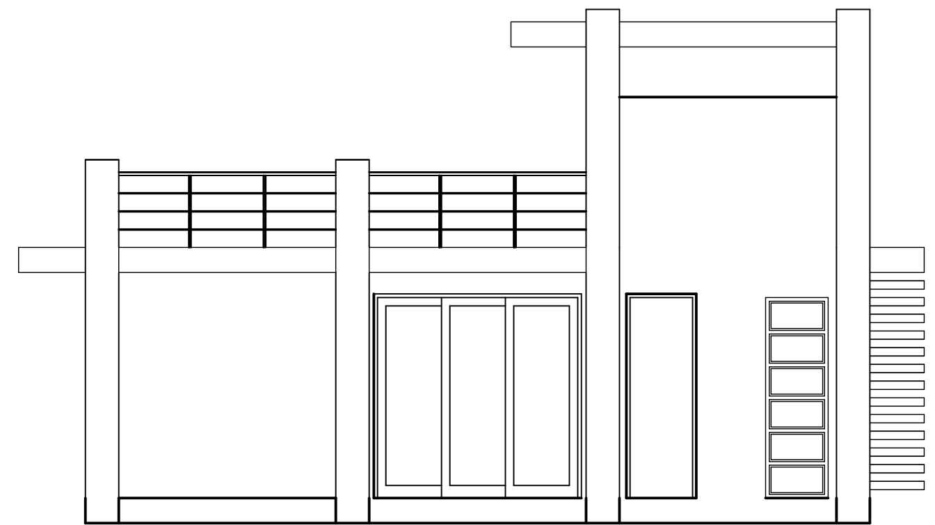
east elevation
